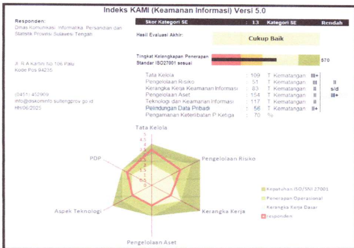
Gambar 1 Dashboard Indeks KAMI versi 5.0
